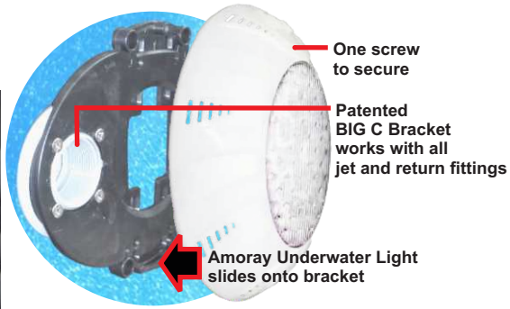
(Above) Example of original light mounting onto C1-12-Thick
